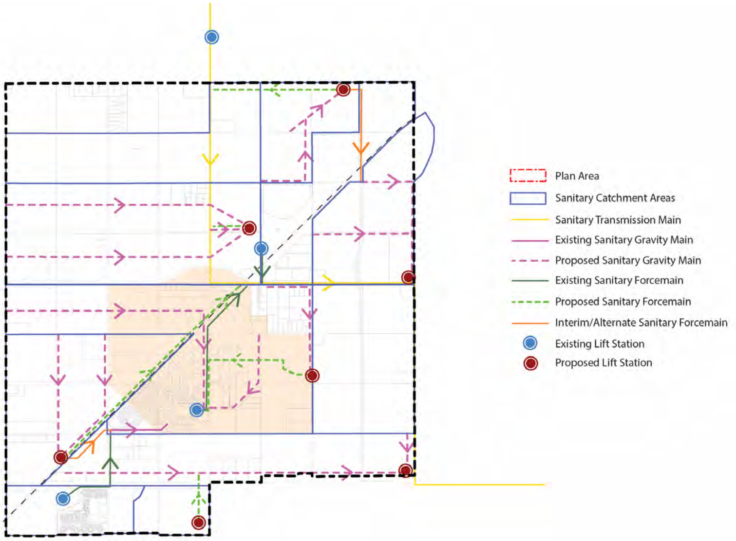
MAP 12 WASTEWATER SERVICING OPTION 1
