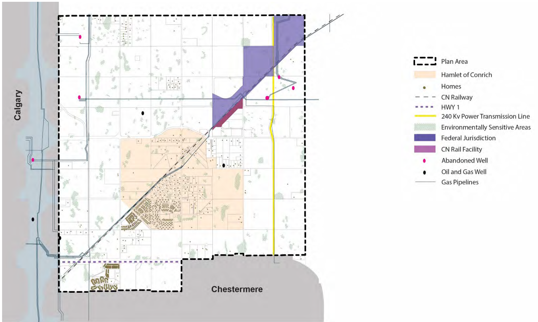
MAP 4 EXISTING CONDITIONS AND UTILITY CORRIDORS
